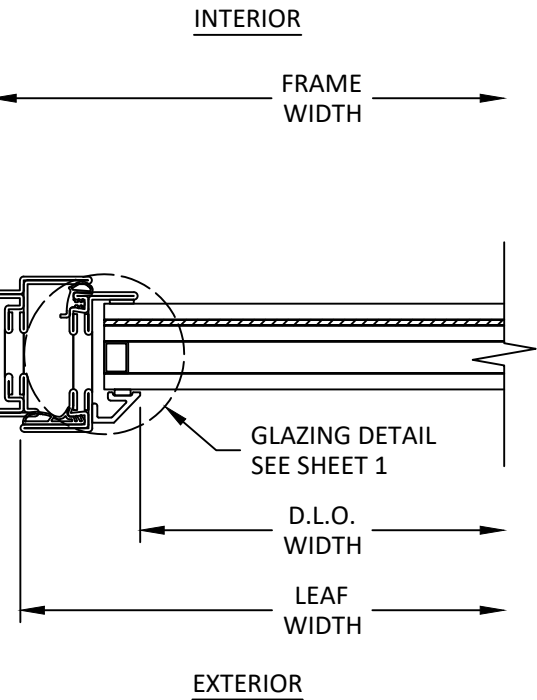
D 6 HORIZONTAL SECTION LOCK JAMB
