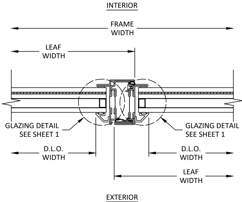
E 6 HORIZONTAL SECTION MEETING STILE
