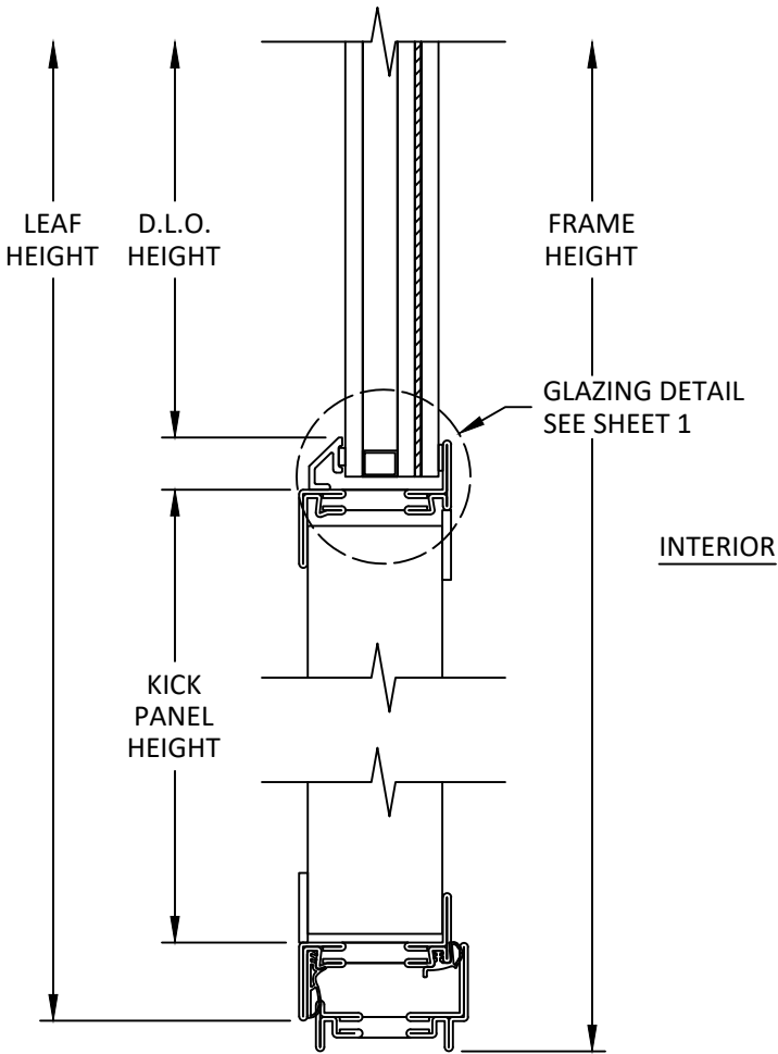
C 5 VERTICAL SECTION SILL WITH KICK PANEL
